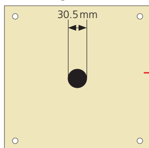
Air rifle target front mask 10m
