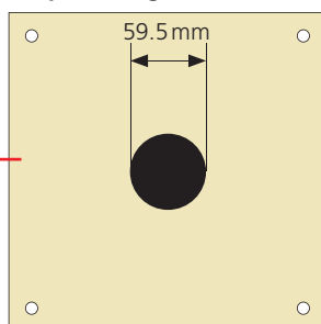
Air pistol target front mask 10m
